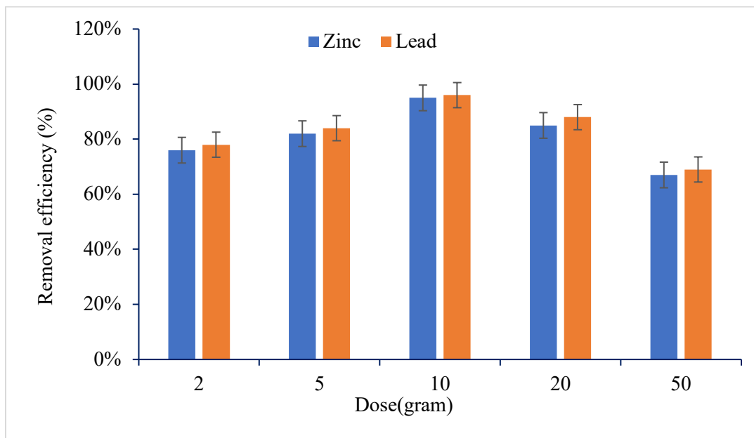
Figure 4: Effect of dose on removal of zinc and lead
