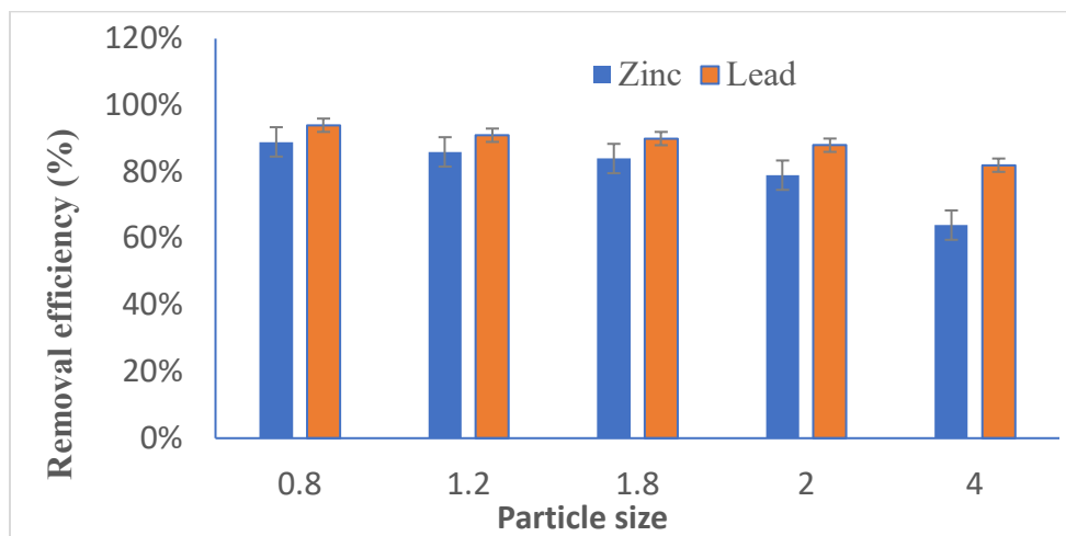
Figure 3: Effect of particle size on removal of zinc and lead
